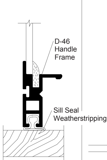
SILL Typical Condition
