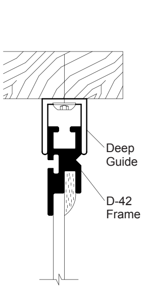
HEAD Typical Condition
