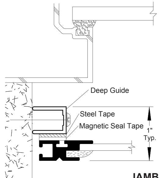
JAMB Mounted to Deep Guide Stop behind Existing Aluminum Framing
