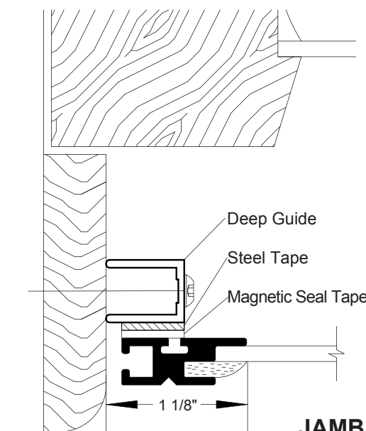
JAMB Mounted on Deep Guide Stop within Wood Double Hung
