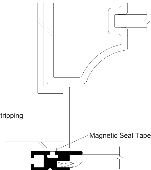
JAMB Mounted on Steel Double Hung
