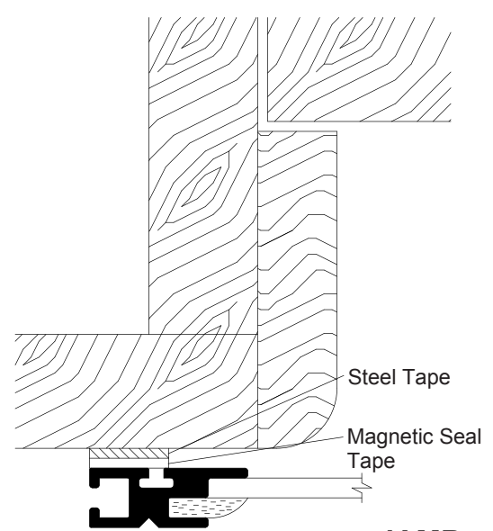
JAMB Overlap Mount on Wood Double Hung
