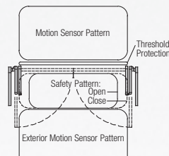
Bifolding Doors
