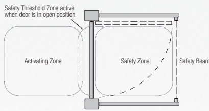
Swinging Doors
