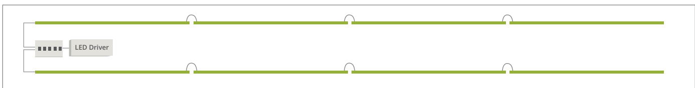
1x8 2 Lamp Model# G2CLA-24-8-X-YY-1K-18 • G2CLA-30-8-X-YY-1K-18 G2CLA-45-8-X-YY-1K-18 • G2CLA-68-8-X-YY-1K-18
