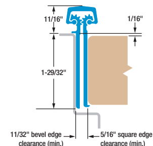
SL24 SD/HD/LL 1/16" door inset. Door edge protector. Frame leaf covers butt hinge preps.
