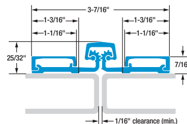
SL60 57" length. Hinge opens to 180°.
