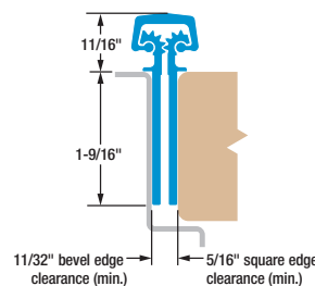
SL11 SD/HD/LL Flush mounted (no door inset).
