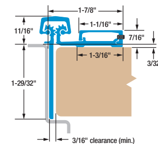
SL54 HD 3/32" door inset. Frame leaf covers butt hinge preps. Tamper-resistant, removable door leaf cover.
