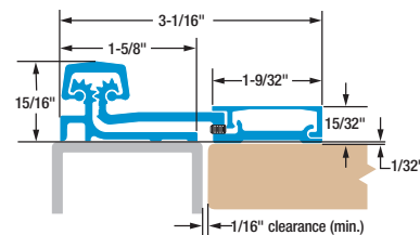
SL21 SD/HD 1/32" door inset. Swing-clear action. Tamper-resistant, removable door leaf cover.
