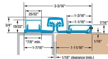
SL57 SD/HD 1/16" door inset. Frame leaf fits narrow (7/8") frame face. Tamper-resistant door leaf cover.
