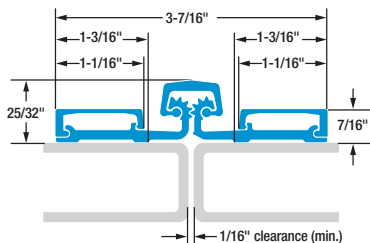
SL60 57" length. Hinge opens to 180°.
