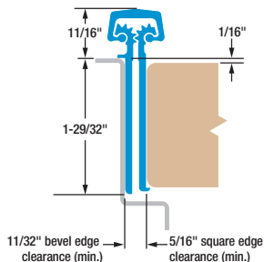
SL24 SD/HD/LL 1/16" door inset. Door edge protector. Frame leaf covers butt hinge preps.
